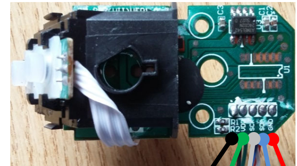
Nunchuk Controller
