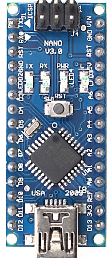
Top View
