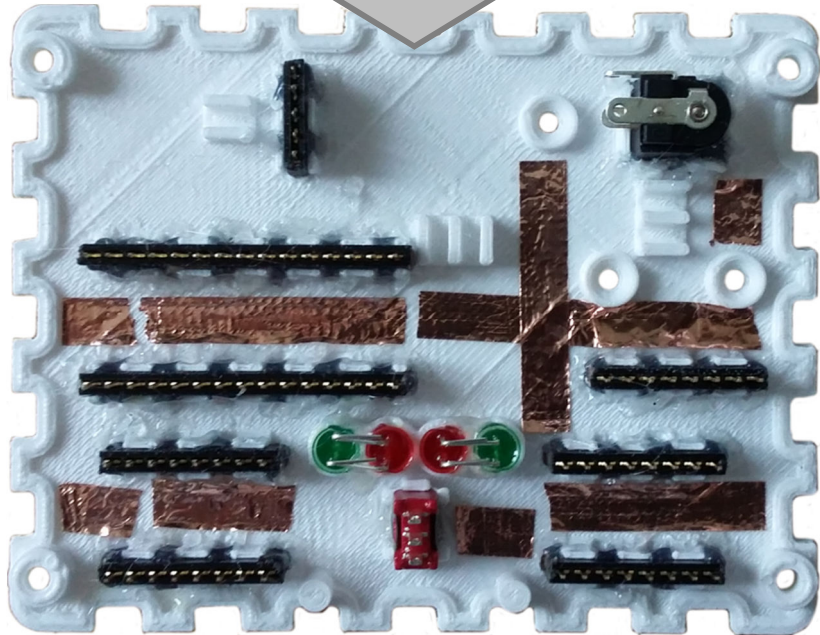
3-D Printed Circuit Mounting Plate
